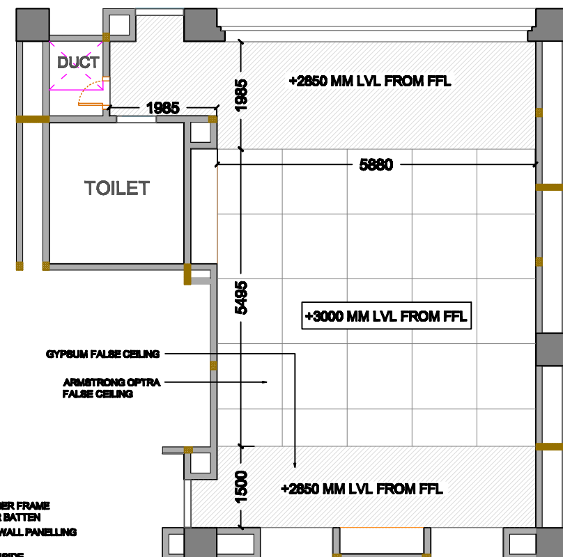
REFLECTED CEILING PLAN LAYOUT
